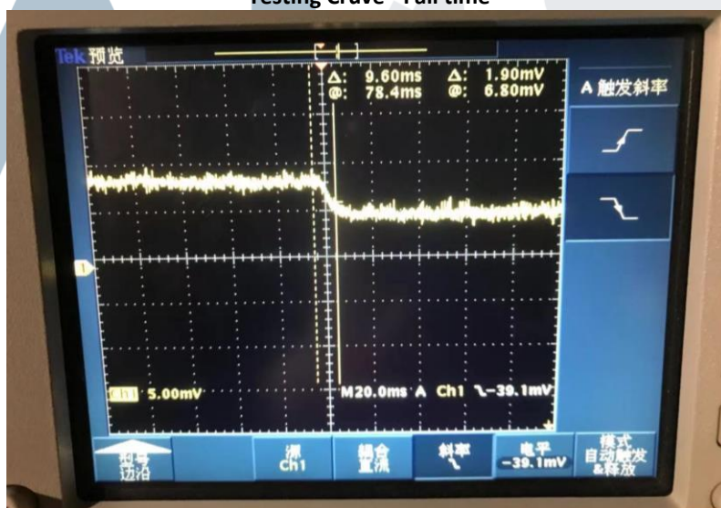
Testing Cruve - Fall time
