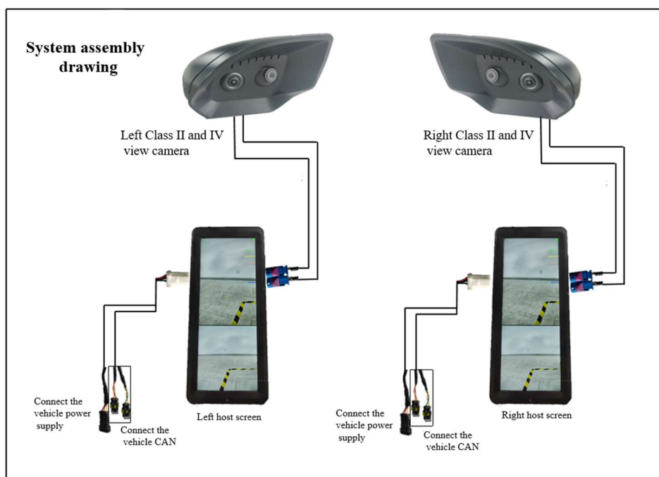
Fig.3 RS-RM2511 System Assembly
